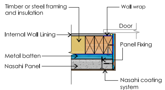
Detail 9.5 Garage Door Jamb Detail
