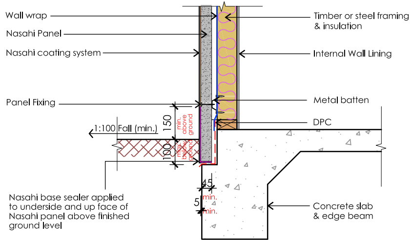
Detail 3.6 Base Panel Detail Below finish ground
