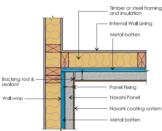
Detail 4.2 Internal Corner Detail
