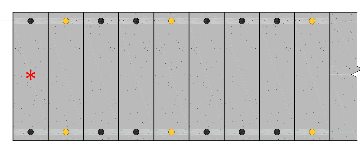
Fig 5.0 Installation Sequence
